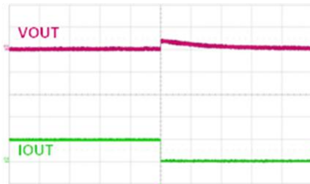
(VOUT: 50mV/div, Iout: 500mA/div, 10ms/div) Vin=3.5V, Vout=2.5V @ Iout=0.5A to 10mA
