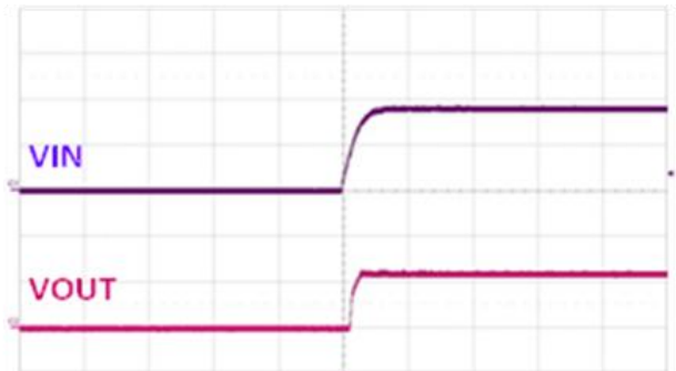
(VIN: 2V/div, VOUT: 2V/div, 1ms/div) Vin=3.5V, Vout=2.5V @ Iout=1A
