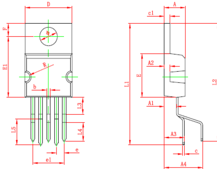
TO-220B PACKAGE OUTLINE DIMENSIONS
