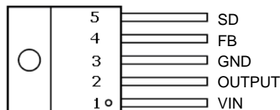
TO-220 5L
