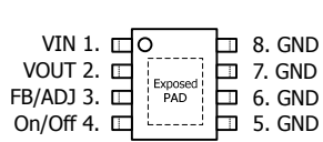
SOP-8PP
