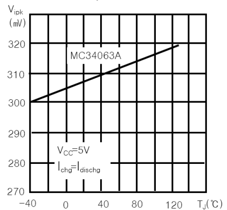
vs. Temperature
